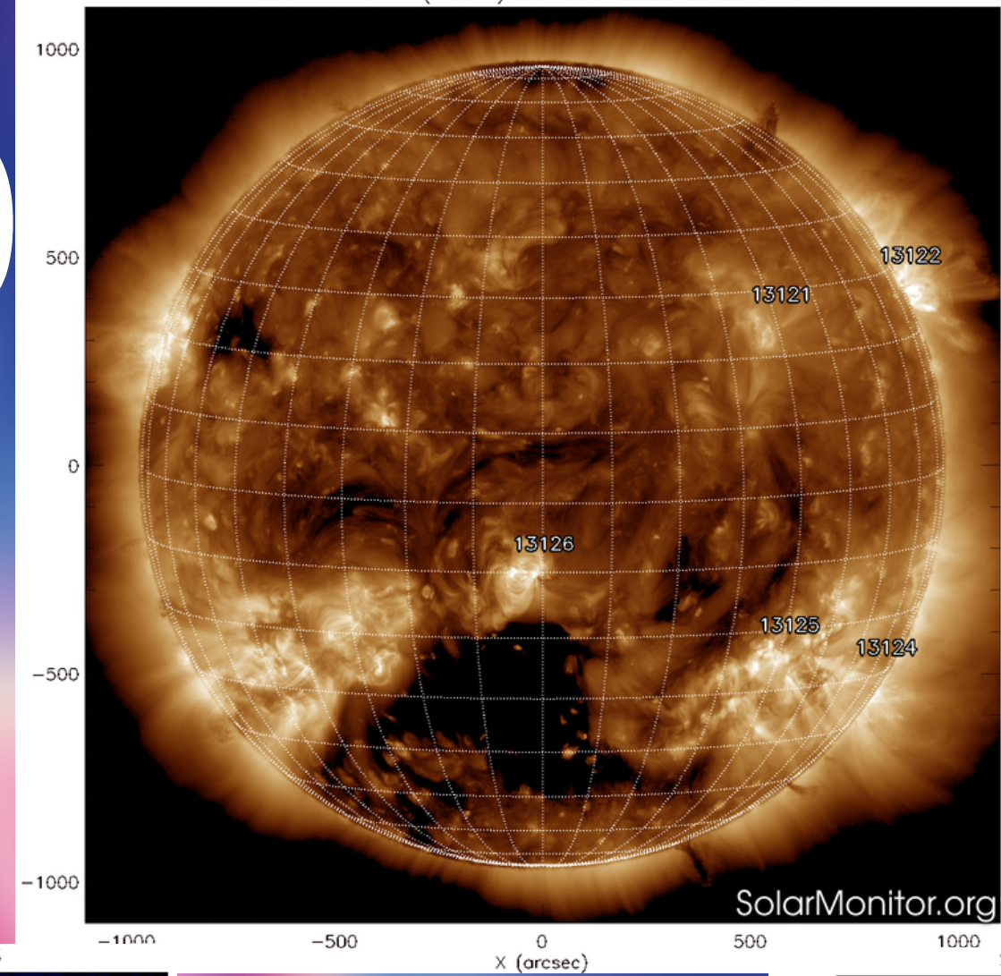
SDO AIA Fe XII (193 Å) 20-Oct-2022 23:25:04.846
