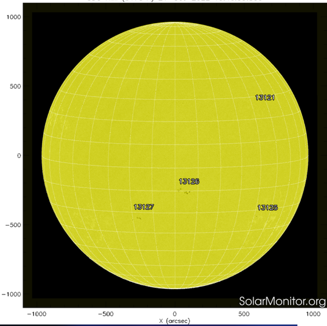
SDO HMI (6173 Å) 21-Oct-2022 10:46:35.800
