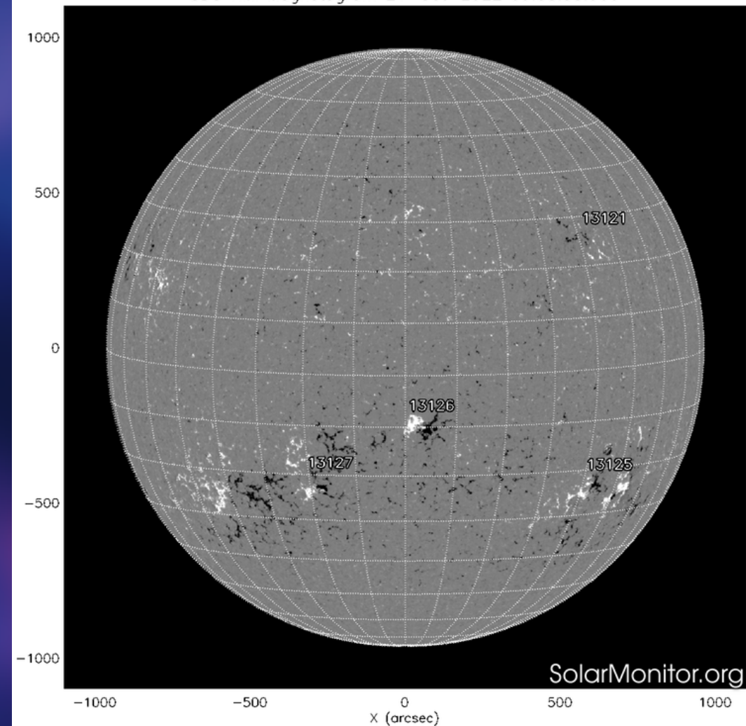
SDO HMI Magnetogram 21-Oct-2022 09:58:35.900
