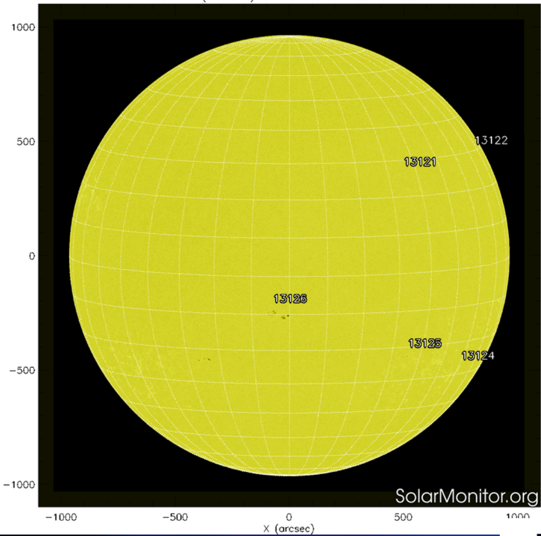
SDO HMI (6173 Å) 20-Oct-2022 22:46:35.800
