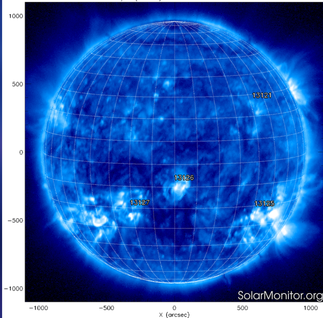
SWAP Fe IX/X (174 Å) 21-Oct-2022 08:55:16.217
