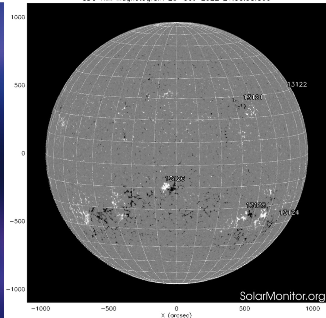
SDO HMI Magnetogram 20-Oct-2022 21:58:35.800
