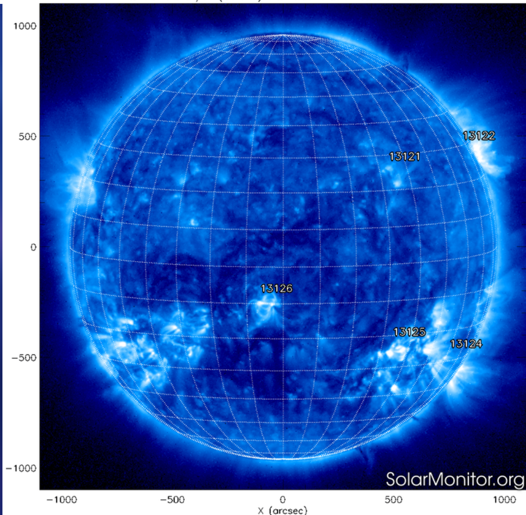
SWAP Fe IX/X (174 Å) 20-Oct-2022 19:51:16.363
