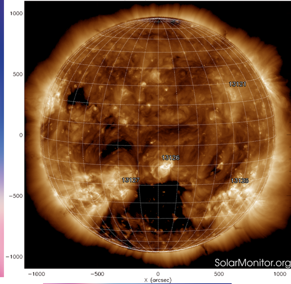
SDO AIA Fe XII (193 Å) 21-Oct-2022 11:24:28.843
